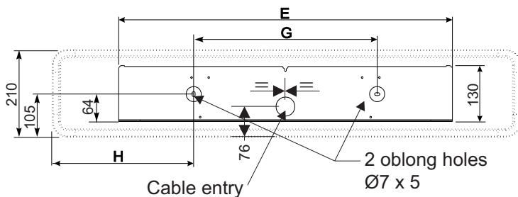
Fixing holes position of wall mounting plate
